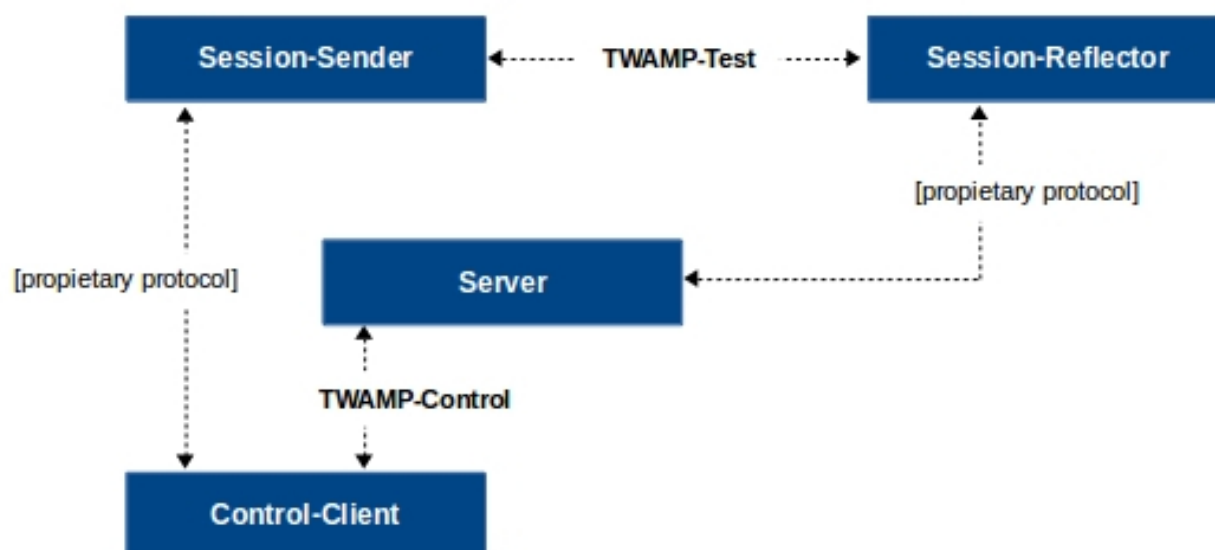
Fig. 1: TWAMP full architecture.
