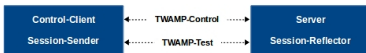
Fig. 2: TWAMP two-hosts model.
