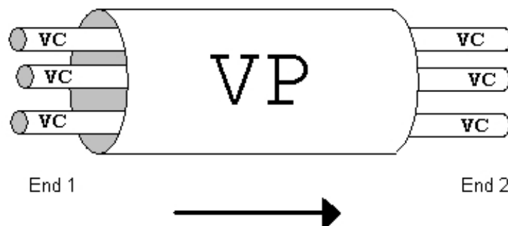
Fig. 2: Grouping of VCs in a VP
