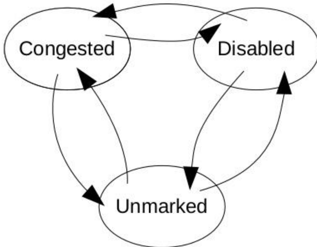
Fig. 3: State diagram
